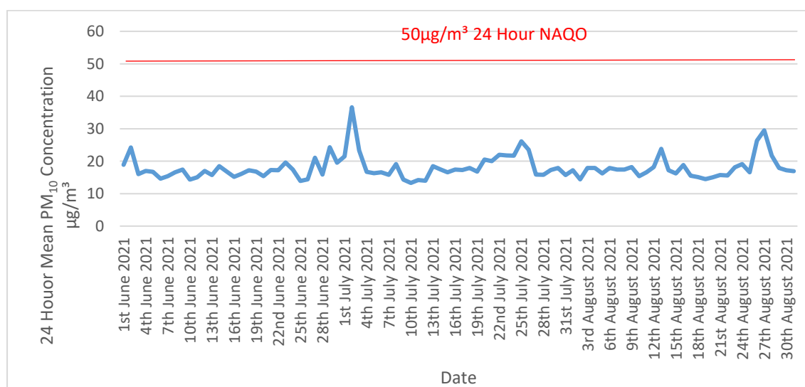
Graph 4: Daily Mean PM 10 Concentrations 1 st June to 31 st August 2021 St Dennis
