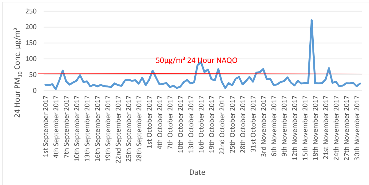
Graph 3: Daily Mean PM 10 Concentrations 1 st September to 30 th November 2017 Nanpean
