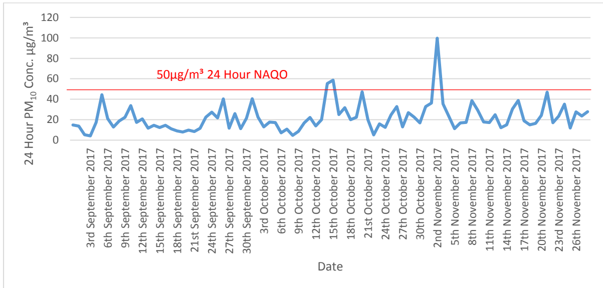
Graph 2: Daily Mean PM 10 Concentrations 1 st September to 30 th November 2017 Treviscoe
