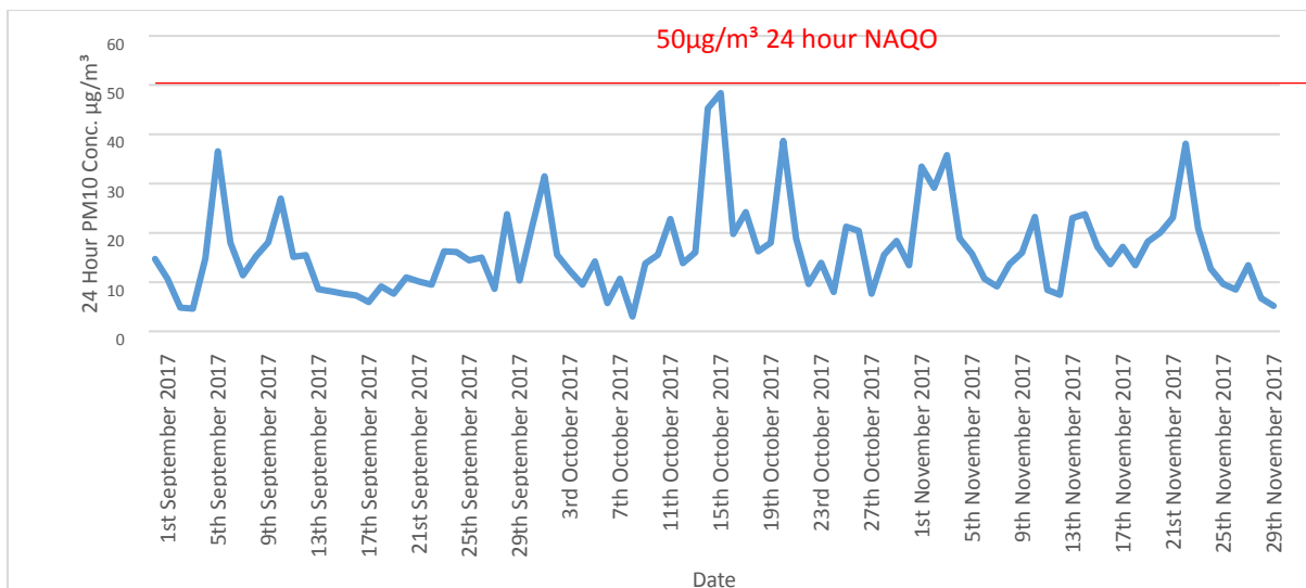
Graph 4: Daily Mean PM 10 Concentrations 1 st September to 30 th November 2017 St Dennis
