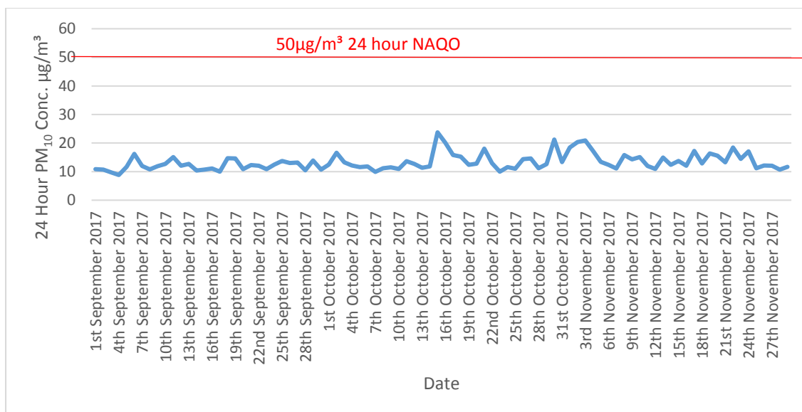
Graph 1: Daily Mean PM 10 Concentrations 1 st September to 30 th November 2017 St Stephen-in-Brannel
