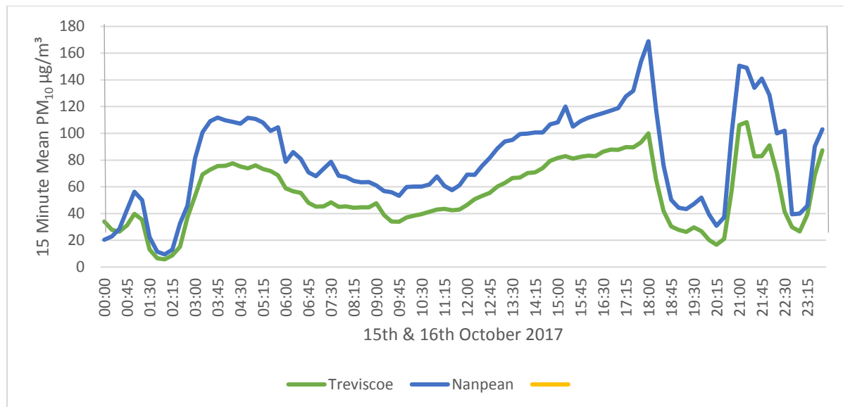
Graph 5: Diurnal PM 10 Concentrations at Treviscoe and Nanpean 15 th and 16 th October 2017
