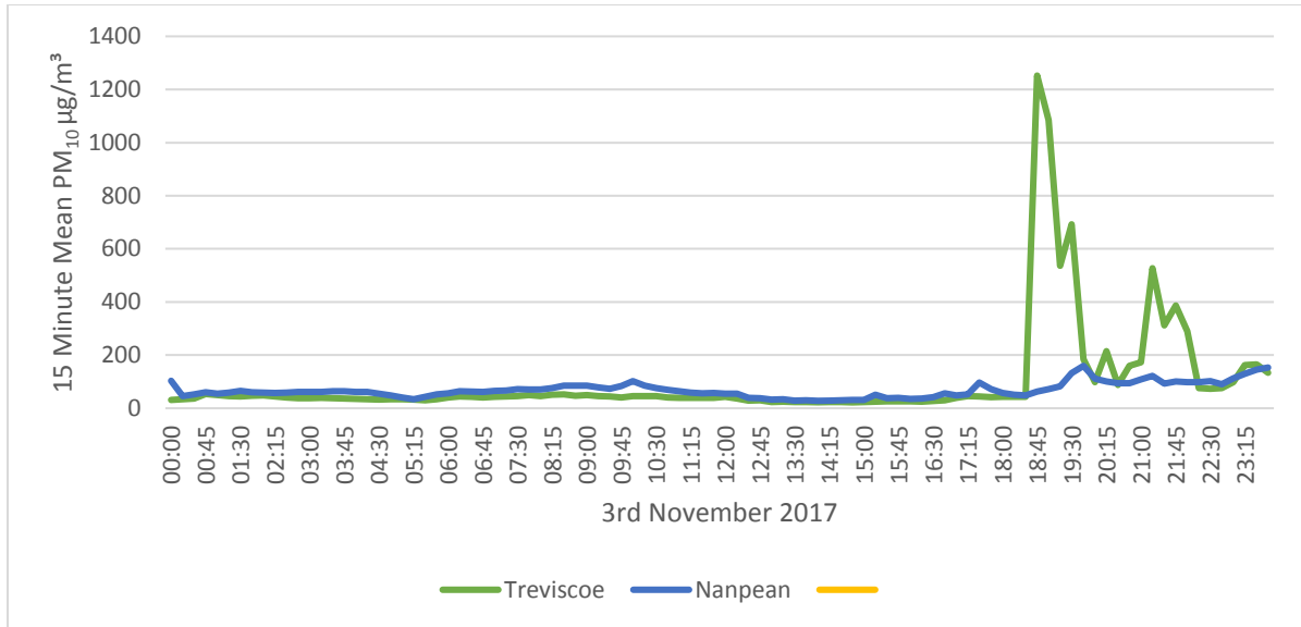
Graph 6: Diurnal PM 10 Concentrations at Treviscoe and Nanpean 3 rd November 2017
